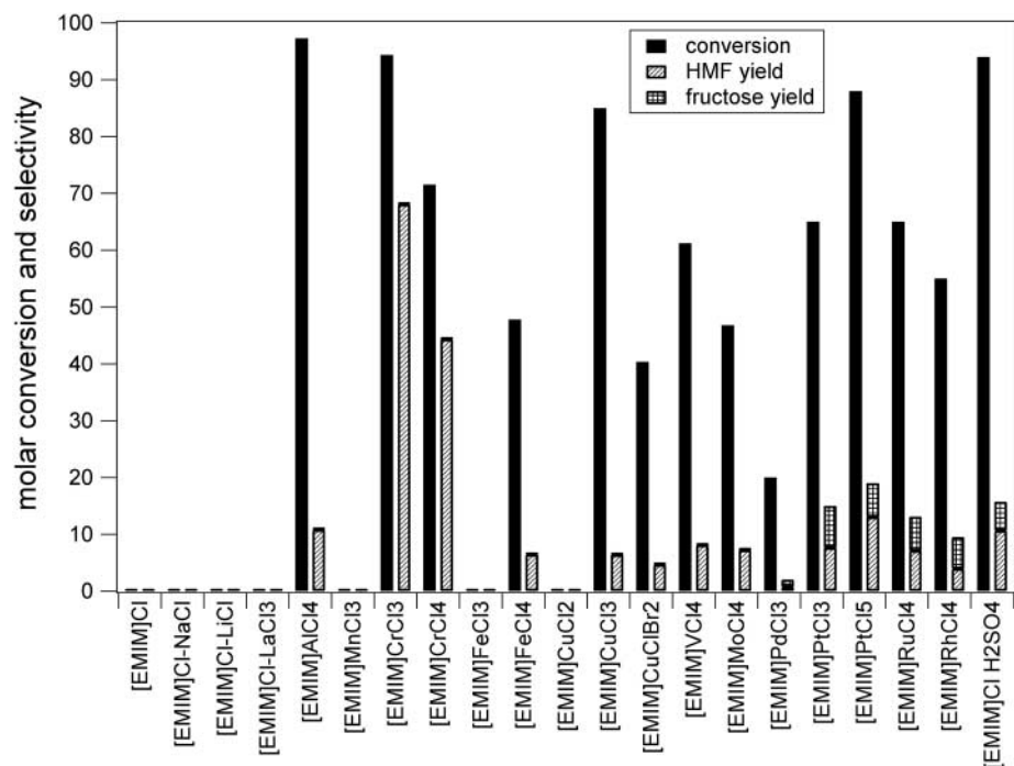
Fig. 3. Glucose conversion in [EMIM]Cl treated with numerous catalysts, most of which are effective for fructose dehydration. Only \text{CrCl}_2 leads to high HMF yield from glucose.
